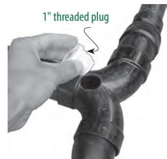
A flow-splitter retrofitted with inspection access. The access is sealed with a threaded plug.
