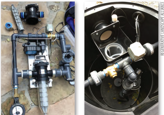
Greywater filter, left; tank and filter, right.
