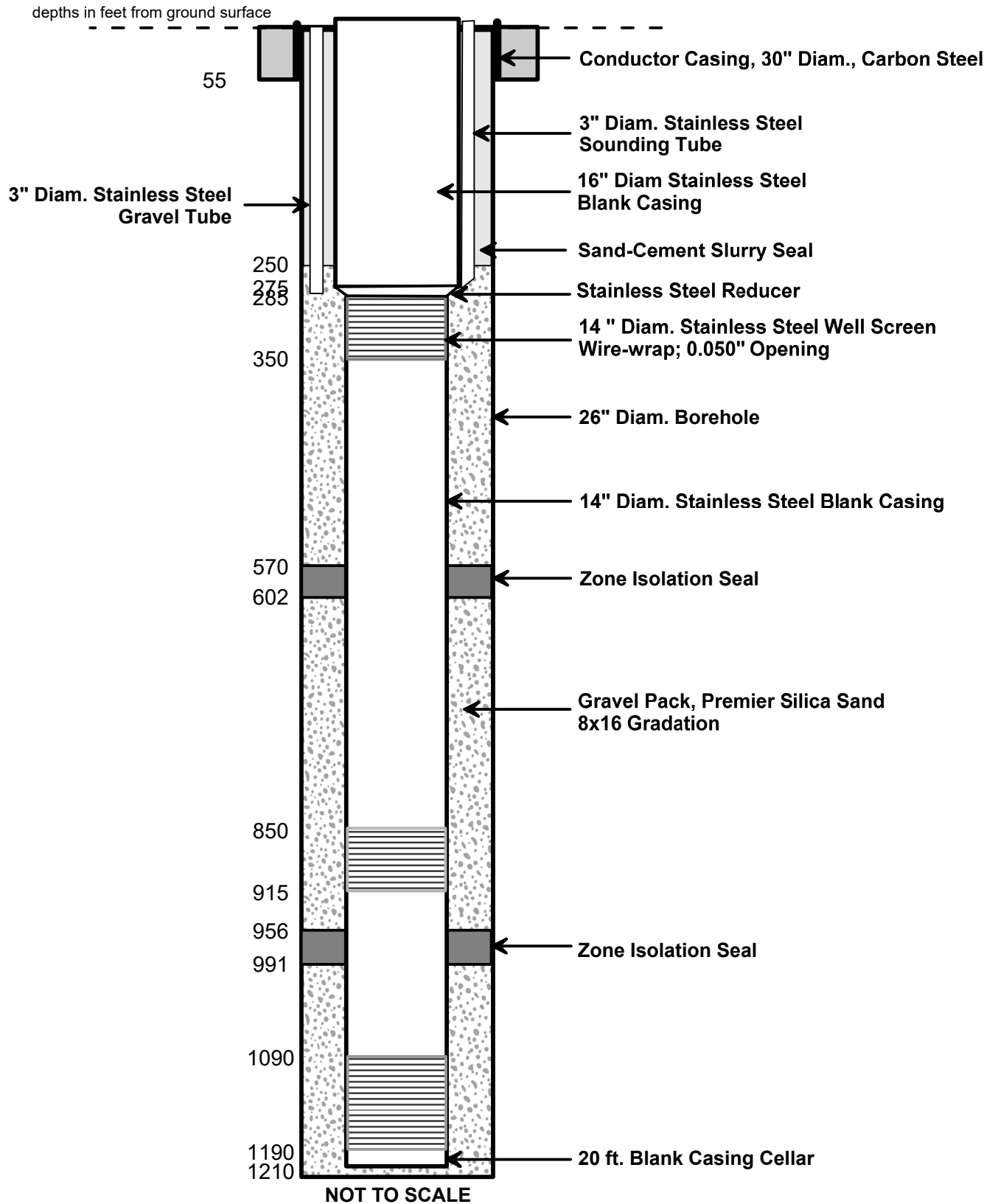
FIGURE 2. EL CARRO WELL #2 DRAWING El Carro Well #2 2023 Rehabilitation Project Carpinteria Valley Water District
