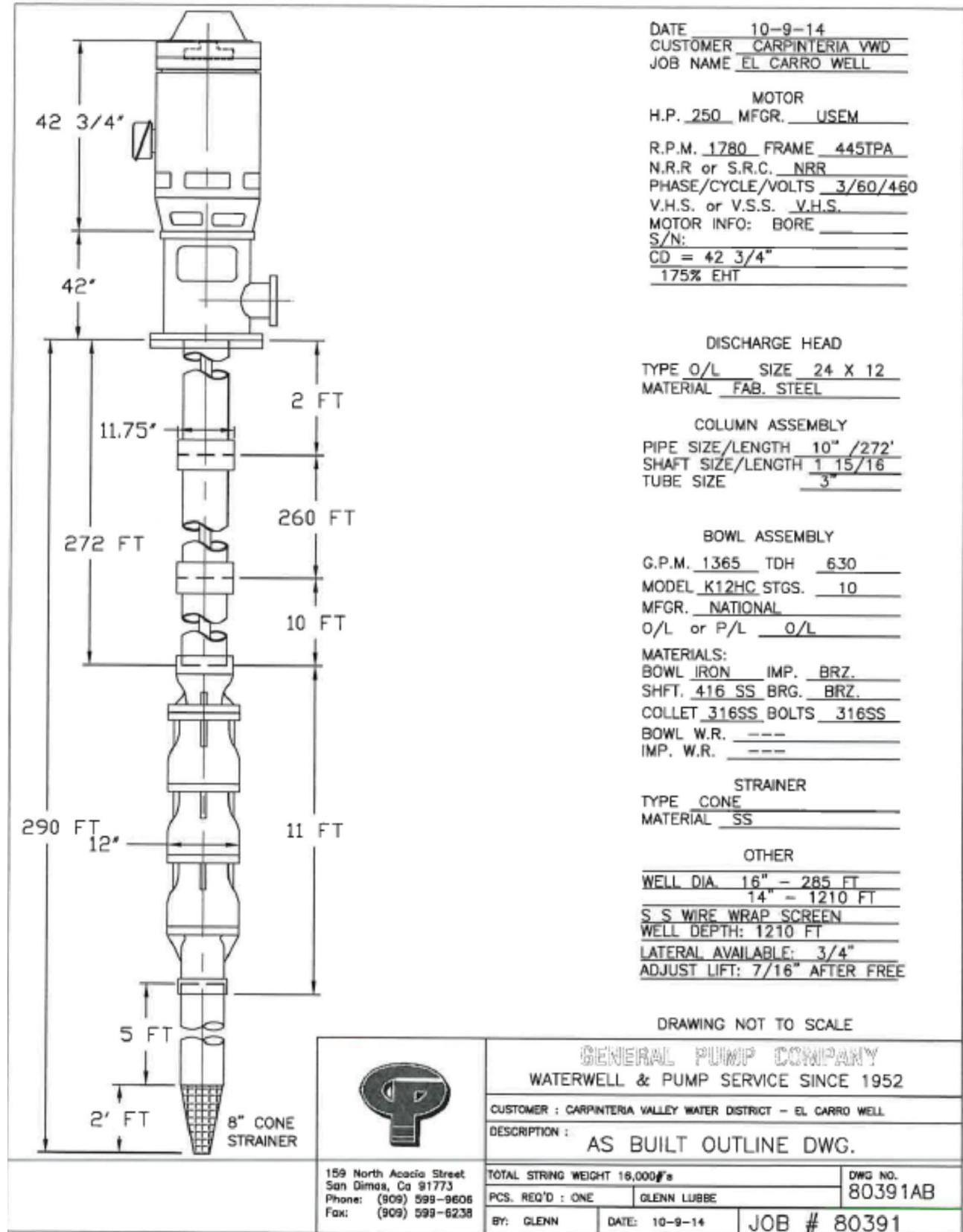
FIGURE 3. EL CARRO WELL #2 PUMP ASSEMBLY El Carro Well #2 2023 Rehabilitation Project Carpinteria Valley Water District
