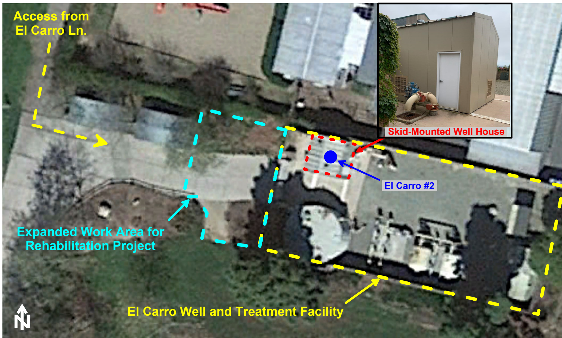
FIGURE 1. EL CARRO WELL #2 SITE MAP El Carro Well #2 2023 Rehabilitation Project Carpinteria Valley Water District
